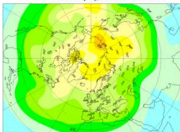
Mean total ozone (DU), 2014/05/01-2014/05/31
